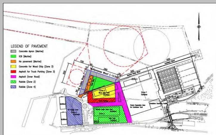
Multi-purpose Terminal development plan
